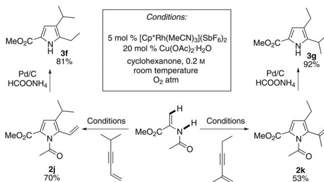
Scheme 6. Preparation of a C2/C3 regioisomeric series.
